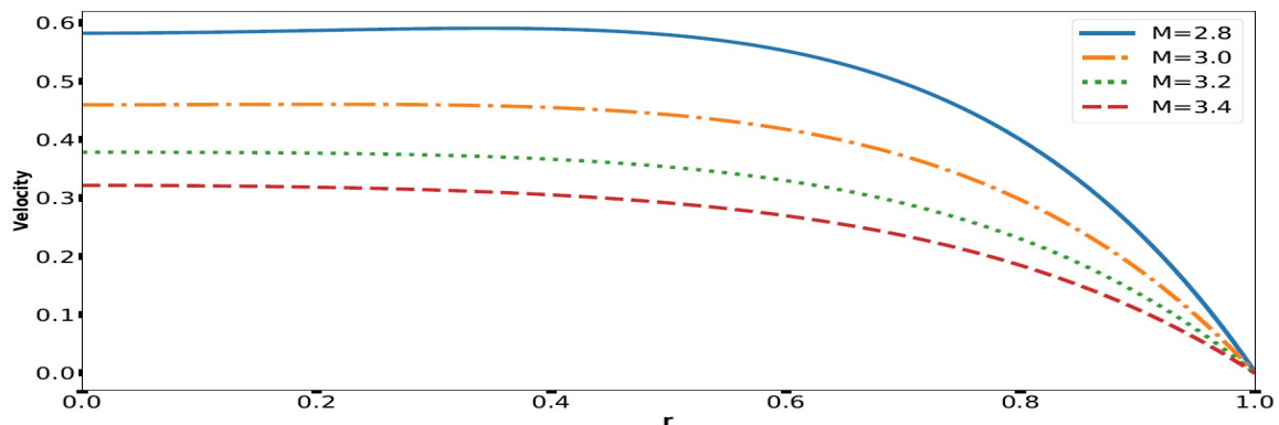
Figure .4: Velocity profiles for M = 2.5 , Gr = 0.05 , \lambda = 188 and different values of Magnetic field parameter, M
