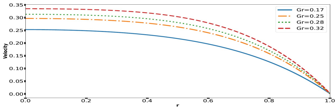
Figure 3: Velocity profiles for M = 1.5 , p = 1 , \lambda = 1000 and different values of Grashof number Gr . In Figure 3, It is clear that an increase in Grashof number increases fluid velocity. This agrees with the results of [11] and [13].
