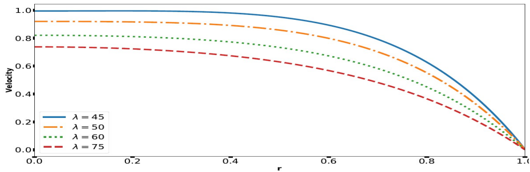
Figure .2: Velocity profiles for Pr = 4 , Gr = 1.0 , \lambda = 180.0 and different values of velocity cooling parameter, \lambda
