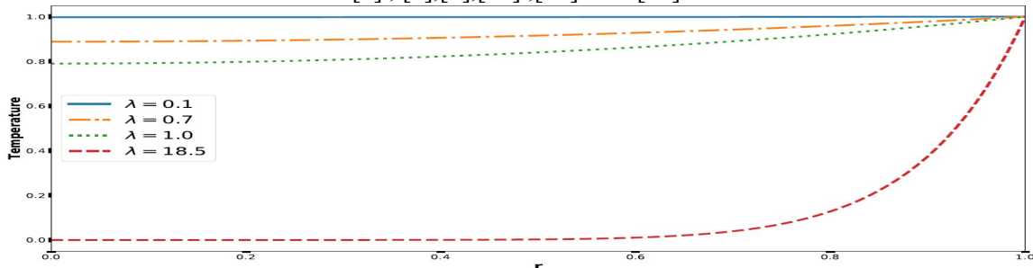
Figure 5: Temperature profiles for with \theta_a = 1.0 and different values of temperature cooling parameter, \lambda
